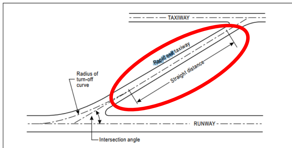
Figure 3-3. Rapid exit taxiway
